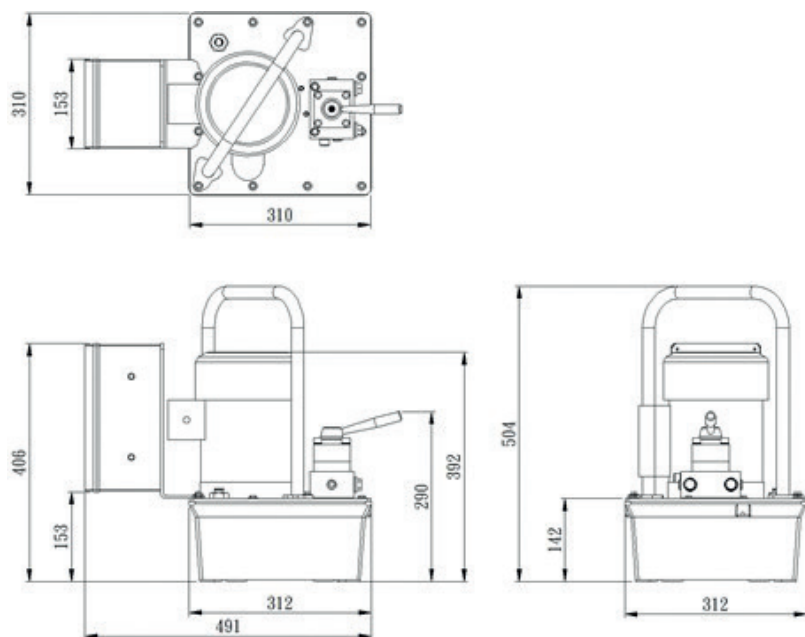
Dimensional drawing EP211
