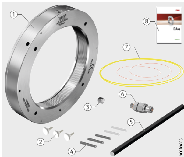
Figura 1 Suministro HYDNUT...-E(-INCH)
